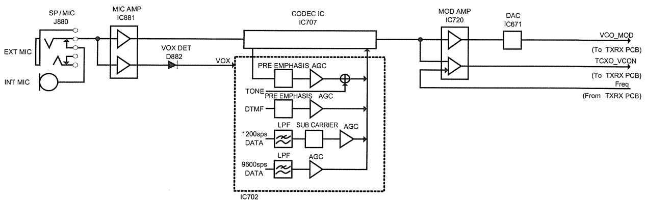
Fig.11 Transmission AF circuit
