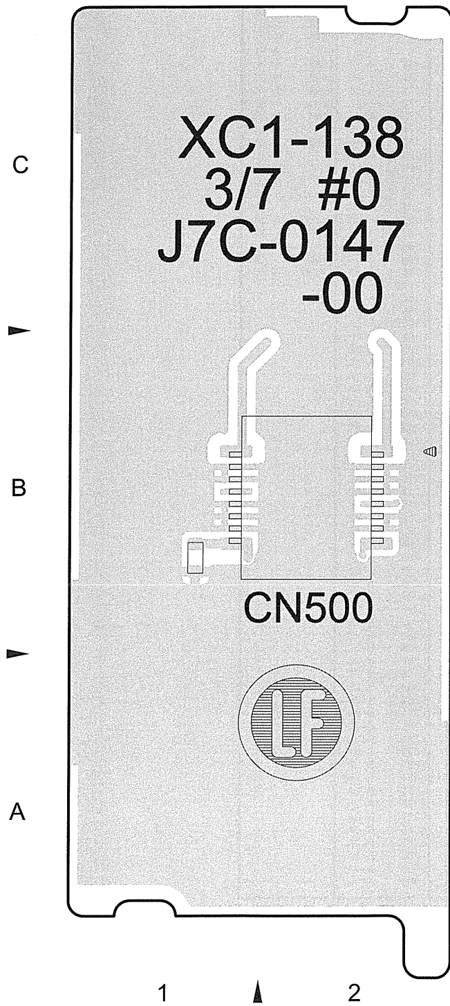
--- Component side view (J7C-0147-00) ---
