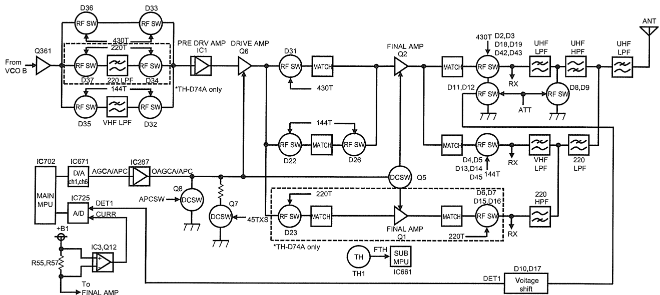
Fig.6 Transmitter circuit
