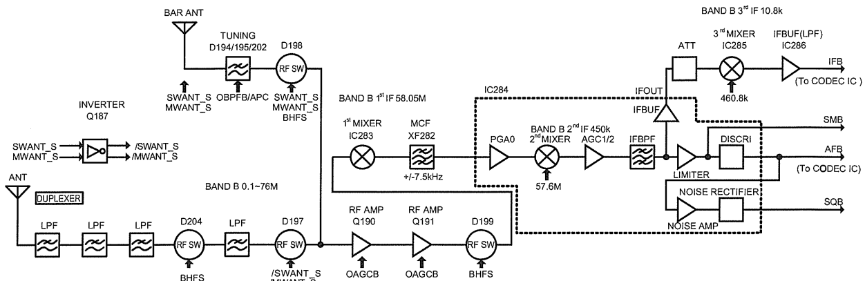
Fig.4 HF receiver circuit
