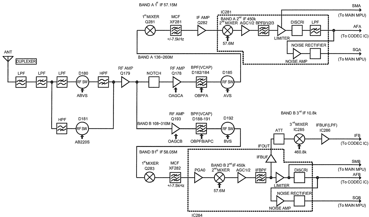
Fig.2 VHF/220MHz receiver circuit
