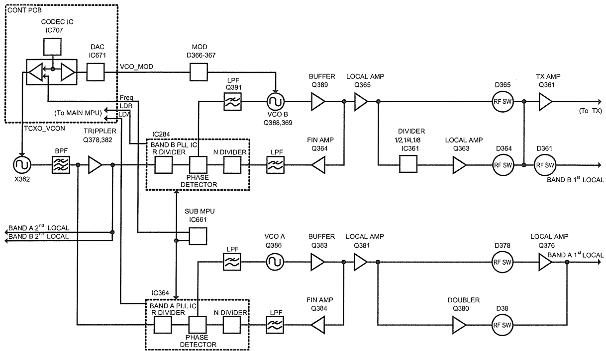
Fig.7 VCO-PLL circuit
