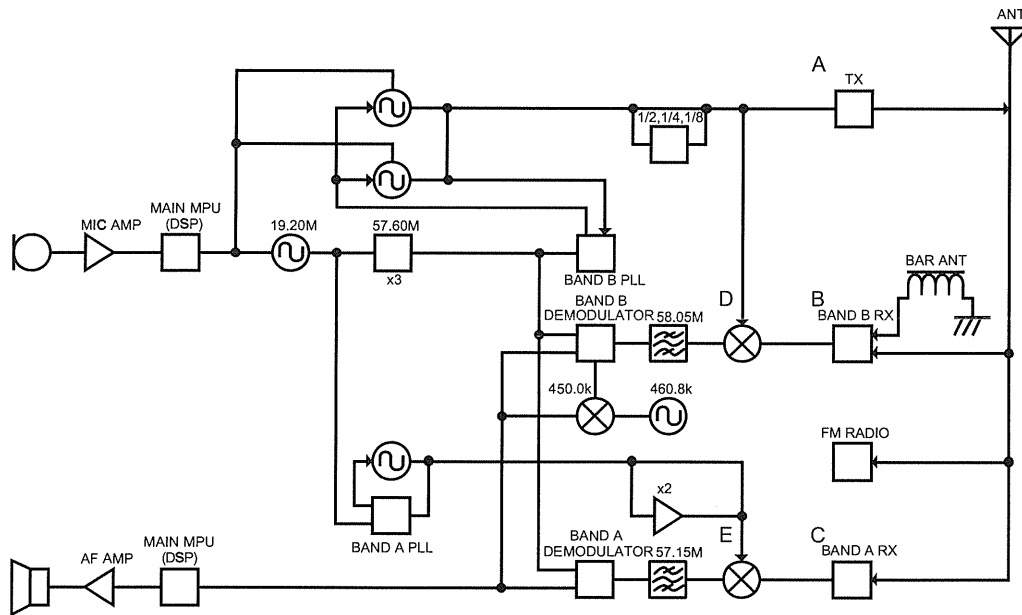
Fig.1 Frequency configuration
