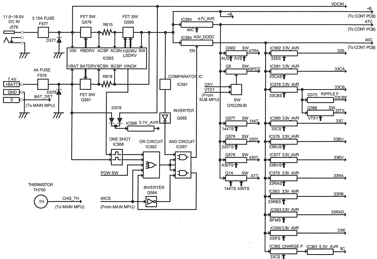
Fig.8 Power supply circuit (TXRX PCB)
