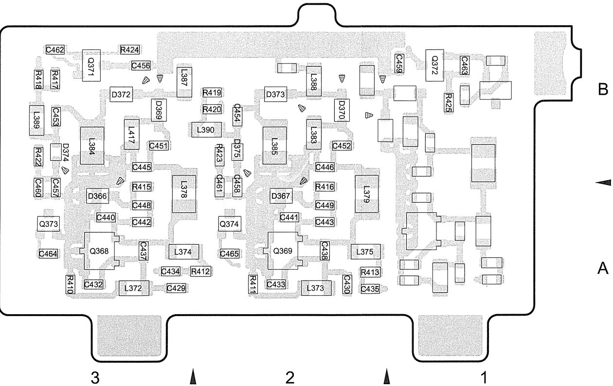
--- Foil side view (J7C-0147-00) ---
