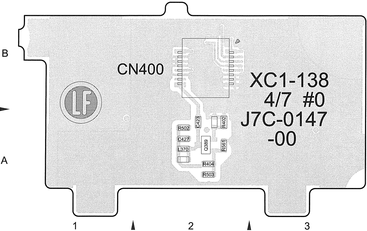
--- Component side view (J7C-0147-00) ---
