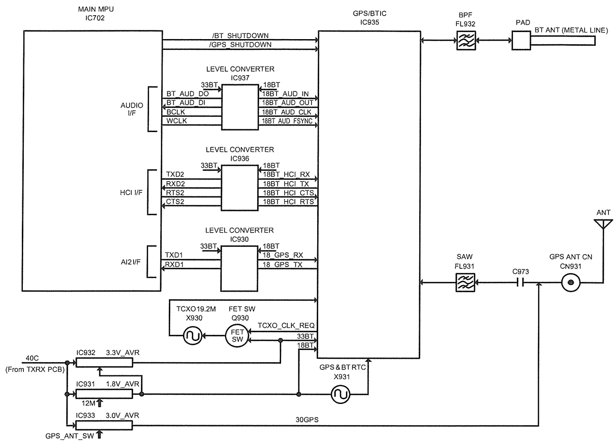
Fig.13 Bluetooth/GPS circuit
