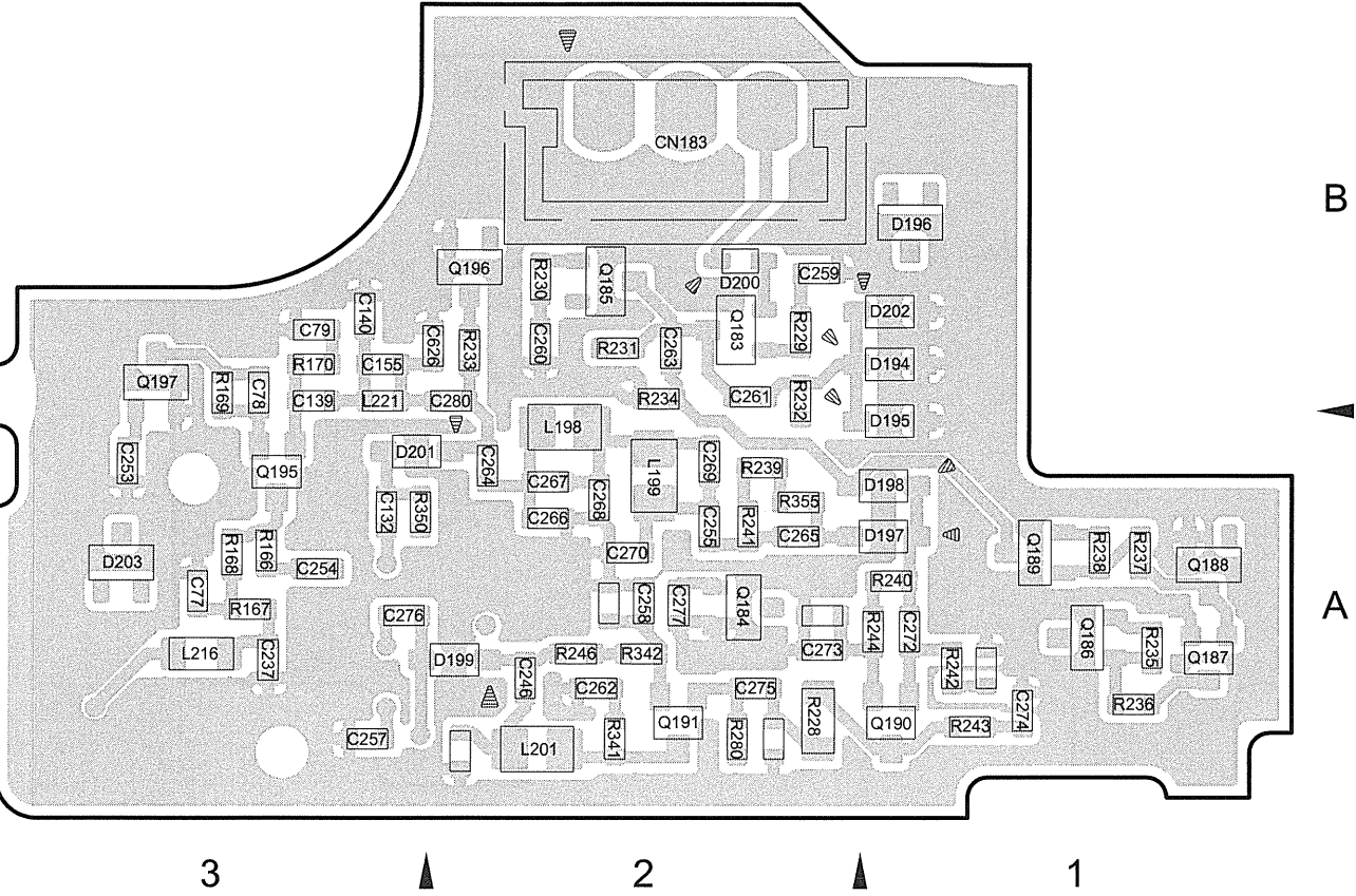
--- Foil side view (J7C-0147-00) ---
