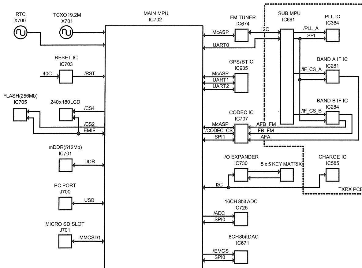
Fig.12 Control circuit
