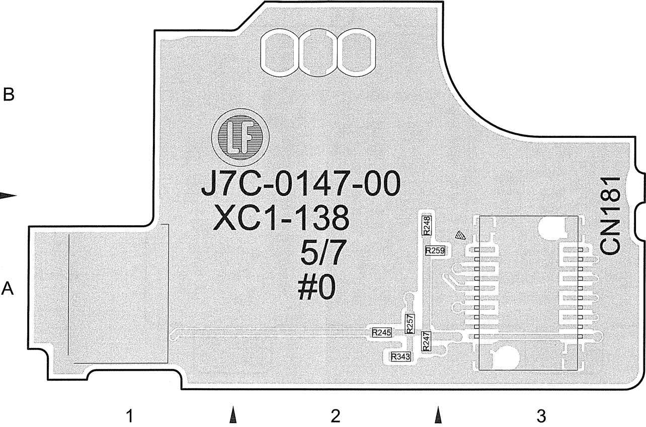
--- Component side view (J7C-0147-00) ---
