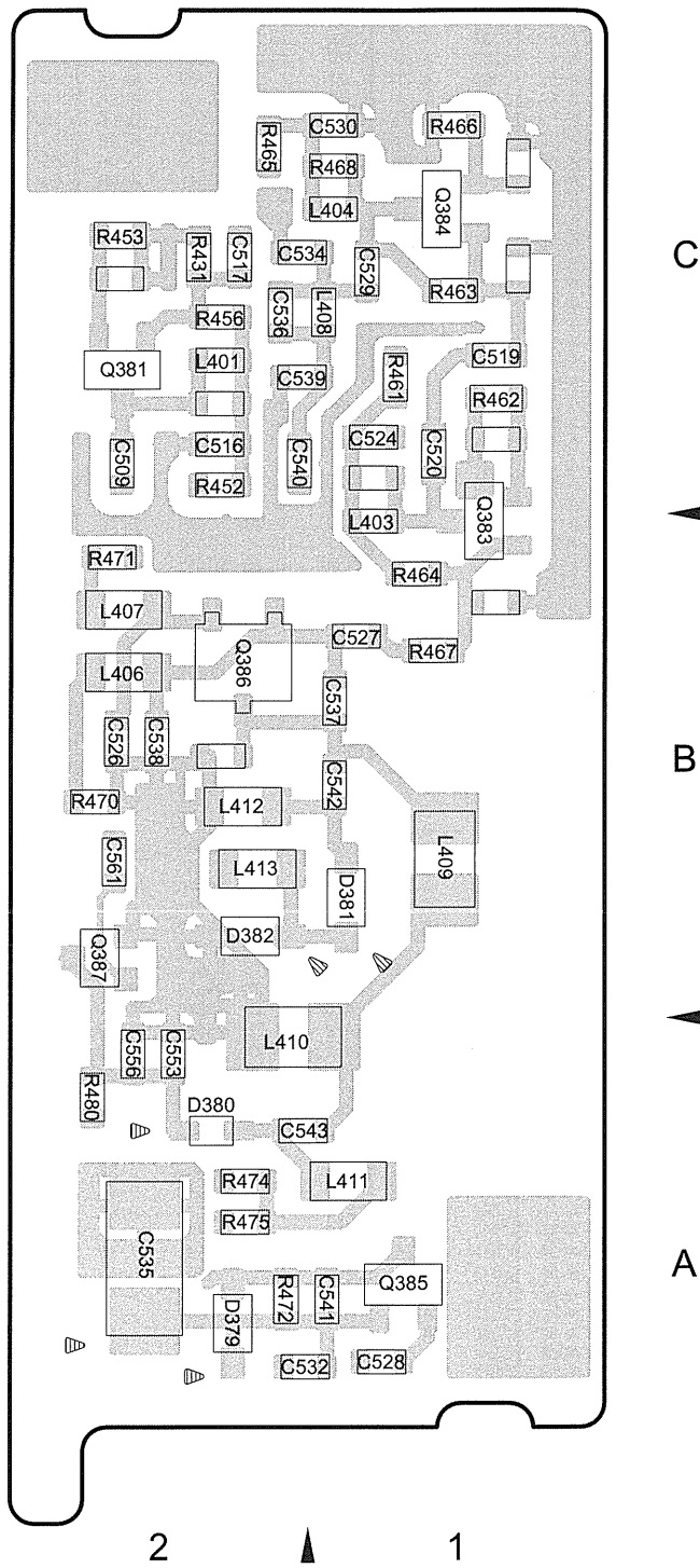
--- Foil side view (J7C-0147-00) ---
